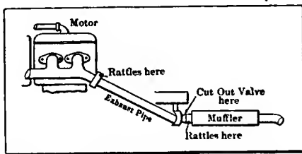
Fig. 3—Illustrating points of leakage in loose exhaust pipe
